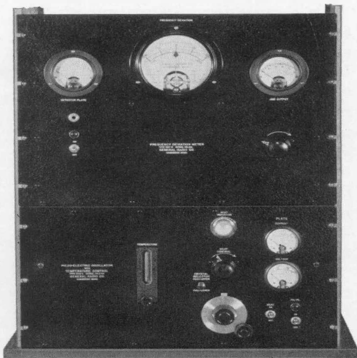
Visual indication of frequency deviation arrived in 1932 in the TYPE 581 Frequency-Deviation Meter
