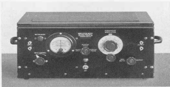
The TYPE 457 Modulation Meter gives laboratory measurement of percentage modulation on positive or negative peaks
