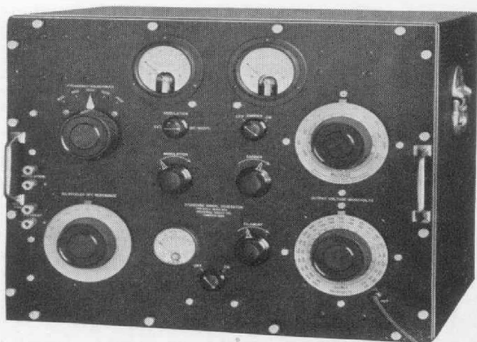
The second step, TYPE 600-A Standard-Signal Generator, for rapid measurements on broadcast receivers at selected frequencies, August, 1931
