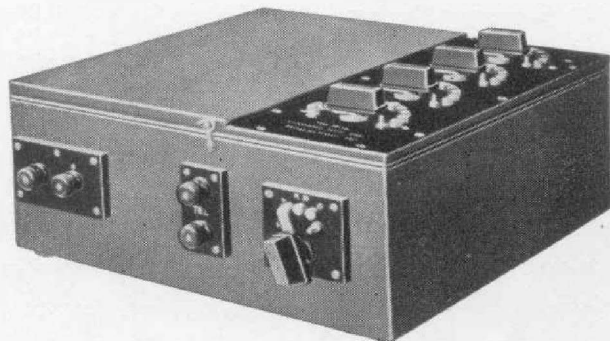
The refinement of decade bridges leads to specialized impedance bridges of greater usefulness in smaller fields, such as the TYPE 216 Capacity Bridge left , and the TYPE 650-A Impedance Bridge right
