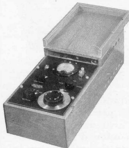
Ten thousand megohms on a bridge! — by means of the vacuum tube used in the TYPE 544 Megohm Meter
