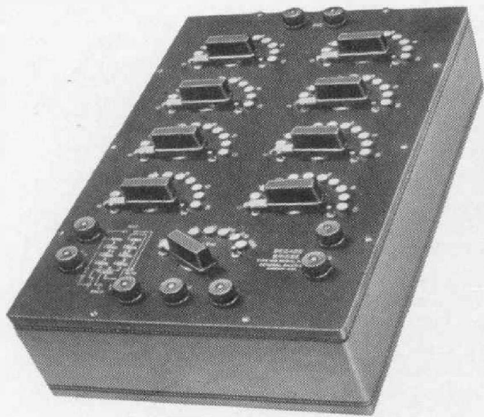
The TYPE 193 Decade Bridge, an intermediate stage in the extension of the decade bridge to alternating-current measurements
