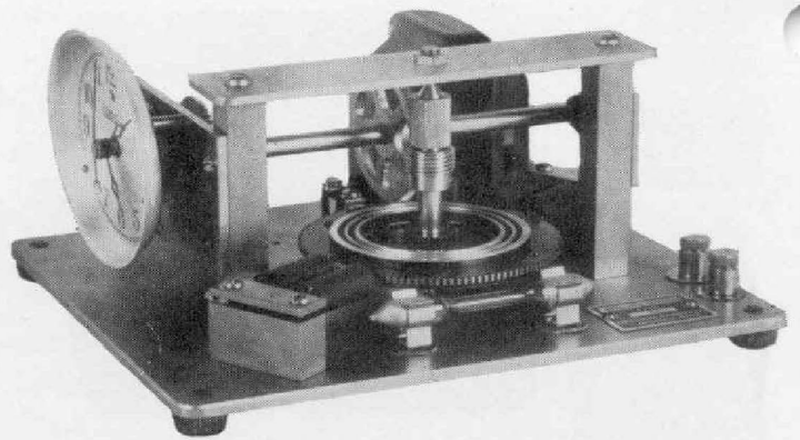
The TYPE 411 Synchronous Motor integrated applied frequencies to give an absolute evaluation in terms of standard time
