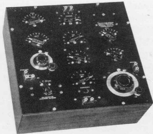
The latest development in measuring small inductances, the TYPE 667-A Inductance Bridge, June, 1935
