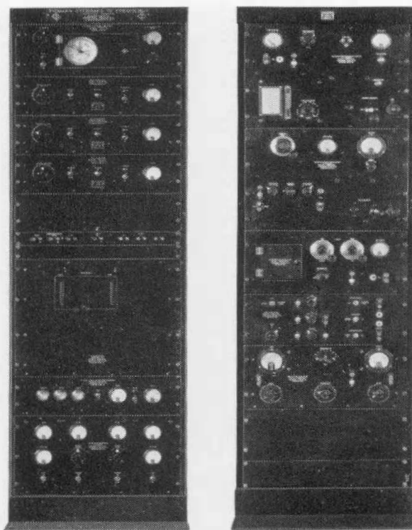
The final development, the Primary Standard of Frequency, accurate to within 5 parts in 10 million, left , and its auxiliary frequency-measuring equipment, right
