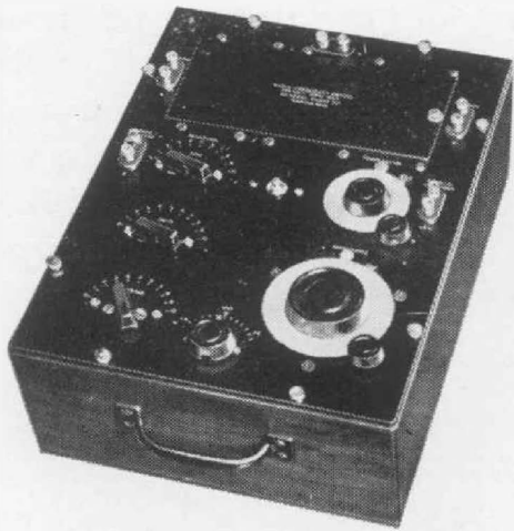
The TYPE 516-C Radio-Frequency Bridge measures impedances directly at frequencies up to 5 megacycles
