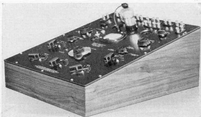
The TYPE 561 Vacuum Tube Bridge has adequately survived all tube developments since its introduction in May, 1932
