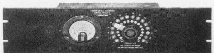
The TYPE 586 Power-Level Indicator program monitors the audio-frequency level fed to the transmitter
