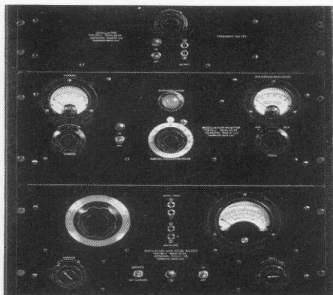
The CLASS 730-A Transmission Monitoring Assembly, introduced January, 1935, permits rapid routine measurement of modulation, distortion, and carrier noise
