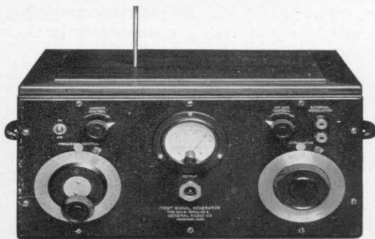
With an eye to the future, the TYPE 604-B Test-Signal Generator for ultra-high-frequency work
