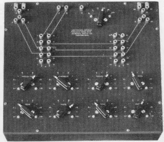
The TYPE 293 Universal Bridge has a greater flexibility of arrangement of the arms and the enclosed-contact construction
